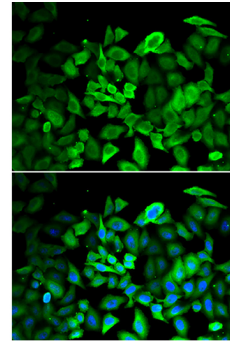
Fig. 4. Immunofluorescence analysis of HeLa cells using ANXA1 antibody. Blue: DAPI for nuclear staining.
