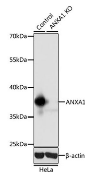
Fig. 2. Western blot analysis of extracts from normal (control) and ANXA1 knockout (KO) HeLa cells, using ANXA1 antibody at 1:1000 dilution. Secondary antibody: HRP-labeled Goat Anti-Rabbit IgG(H+L) (A0208) at 1:1000 dilution. Lysates/proteins: 25µg per lane. Blocking buffer: QuickBlock™ Blocking Buffer (P0231). Detection: BeyoECL Star (P0018A). Exposure time: 1s.
