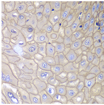
Fig. 3. Immunohistochemistry of paraffin-embedded human esophagus using ANXA1 antibody at dilution of 1:100 (40x lens).
