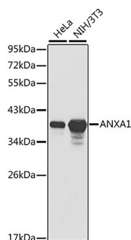
Fig. 1. Western blot analysis of extracts of various cell lines, using ANXA1 antibody at 1:10000 dilution. Lysates/proteins: 25µg per lane. Blocking buffer: QuickBlock™ Blocking Buffer (P0231).
